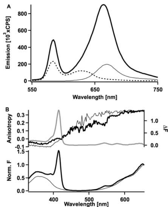
Figure 5. Fluorescence emission (A, \lambda_{\text{ex}} = 415 nm), excitation and anisotropy spectra (B, \lambda_{\text{em}} = 675 nm) of the bichromophorylated ZnMP→PCB systems in HP7::ApcE \Delta . (A) PCB-chromophorylated (thin line), and ZnMP in PCB-chromophorylated and non-chromophorylated (thick dotted and solid lines, respectively) (B) Top: PCB anisotropy spectra of proteins with or without ZnMP (thin and thick black lines, respectively) and difference between their normalized excitation spectra (grey line). Bottom: PCB excitation spectra of proteins with or without ZnMP (thin and thick lines, respectively) normalized at 654 nm (640 nm, for ApcE \Delta N ::HP7::ApcE \Delta C ).
