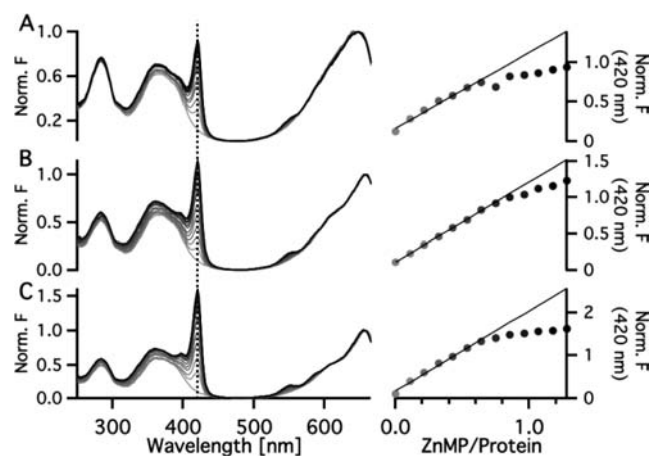
Figure 6. Left: Fluorescence excitation spectra of the bichromophorylated ZnMP→PCB systems ApcE \Delta N ::HP7::ApcE \Delta C (A), ApcE \Delta ::HP7 (B), and HP7::ApcE \Delta (C) titrated with ZnMP. Emission is detected at 675 nm and the spectra are normalized at the red-most excitation peak of PCB (646 nm for HP7::ApcE \Delta ::HP7, and 658 nm for ApcE \Delta ::HP7 and HP7::ApcE \Delta ). The dashed line marks the excitation band at 420 nm that is due to EET from ZnMP to PCB. Right: Saturation binding curves were constructed by plotting the band's intensity as a function of ZnMP to protein molar ratios.
